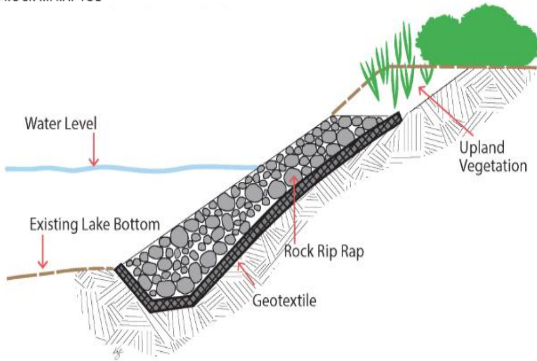
FIGURE 9: ROCK RIPRAP TOE
